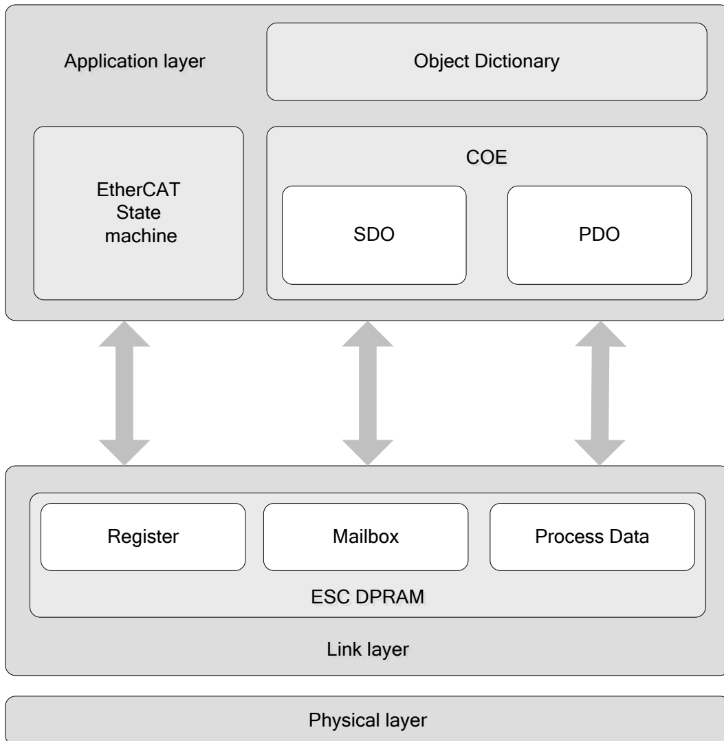
Figure3-1 Communication structure
