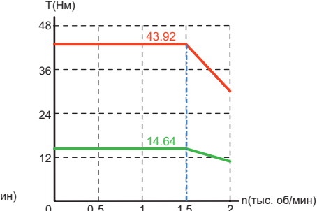
V7E-M13 □-2R315-□ □ L
