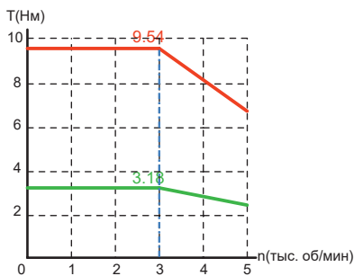
V7E-L08A-1R030-□□
