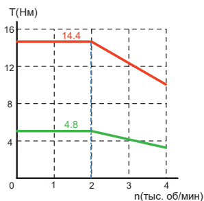
V9E-L13D-3R020
