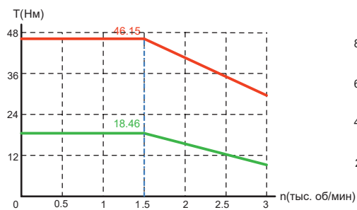
V7E-M18-2R915-□□H
