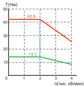
V9E-M13D-3R020
