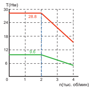
V9E-M13D-2R020
