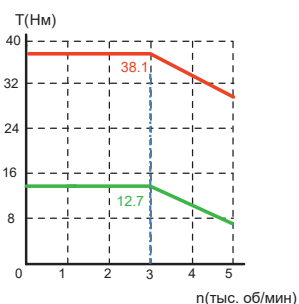
V9E-L13D-4R020
