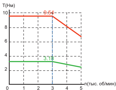
V7E-L08A-1R030-□□
