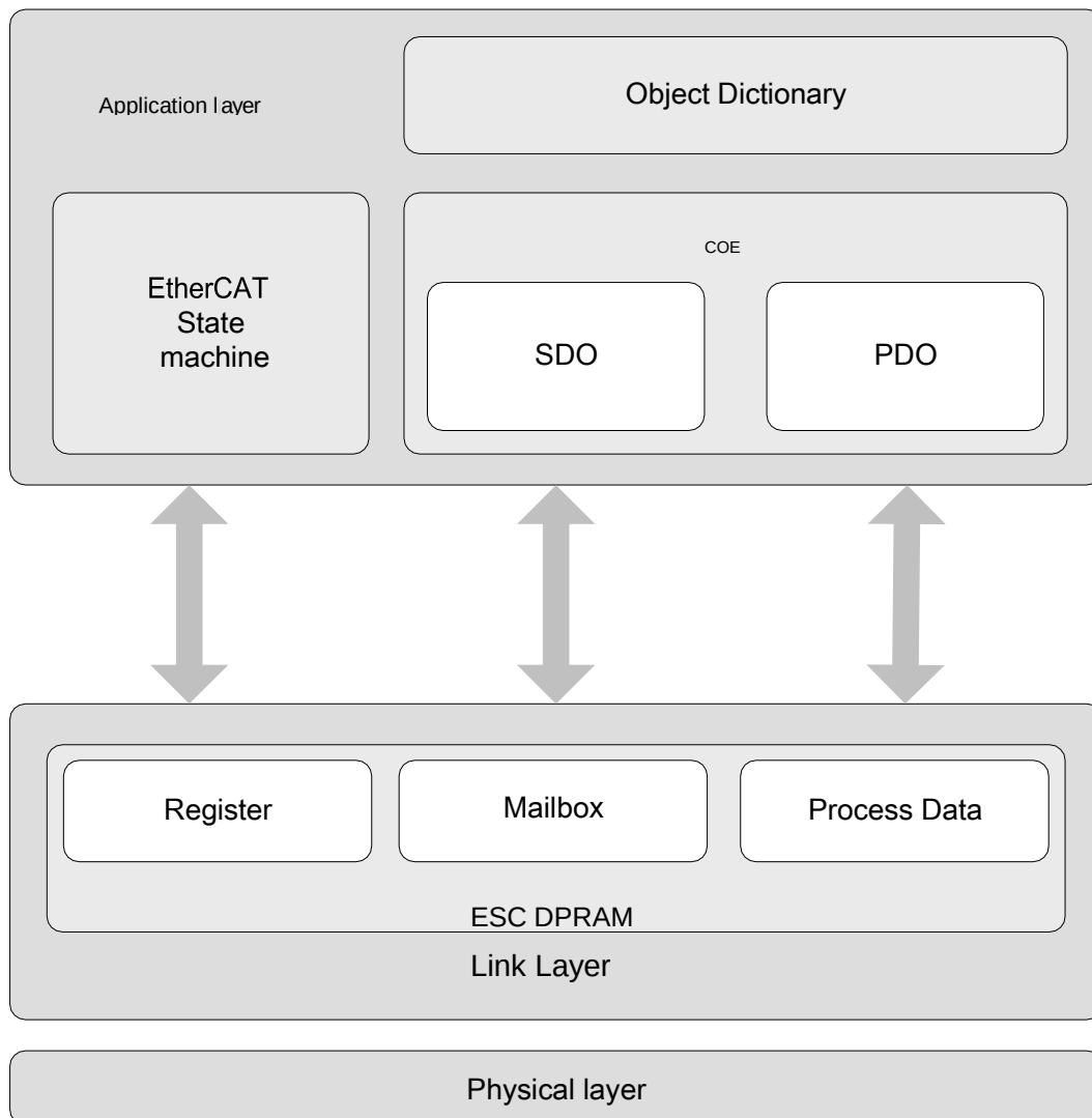
Figure3-1 Communication structure
