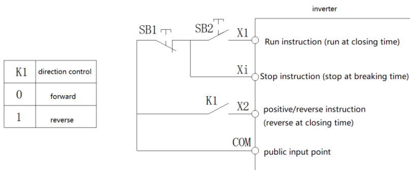
Schematic diagram of three-wire system control 1
