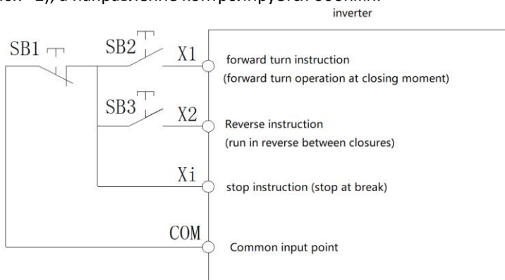
Three-wire system control 2 schematic diagram
